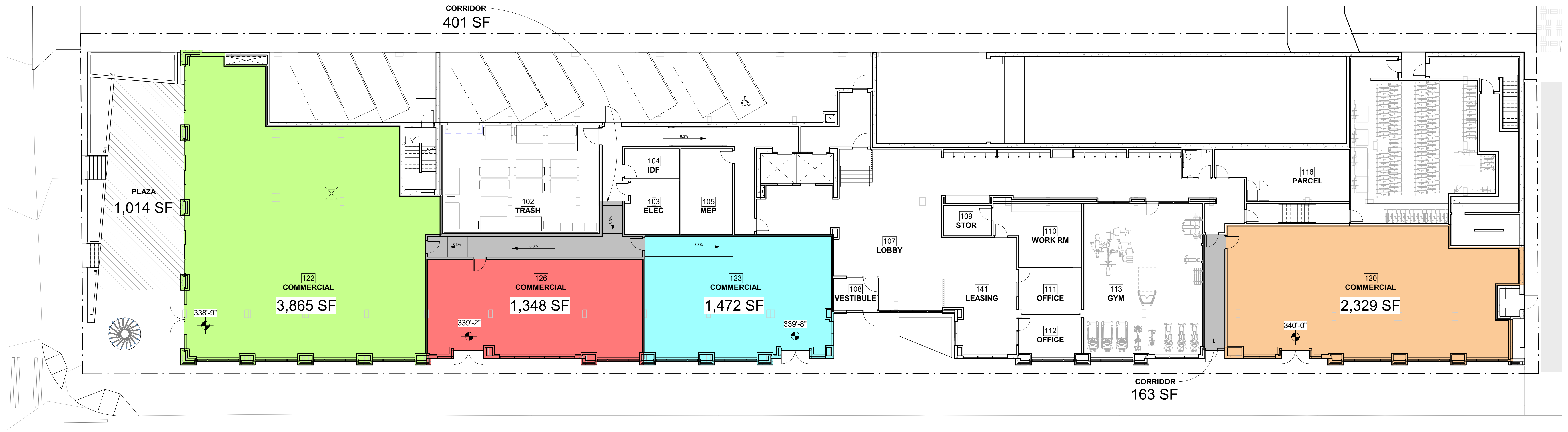
1 A10.00 LEVEL 1 RETAIL AREA PLAN SCALE: 3/32" = 1'-0"
