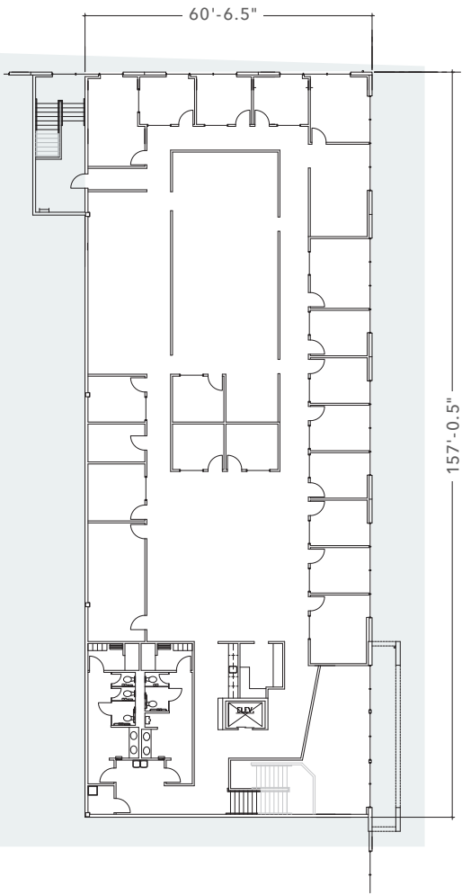
SECOND FLOOR
